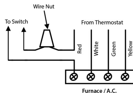
Figure 2: Wiring Diagram for Unit Shutdown
