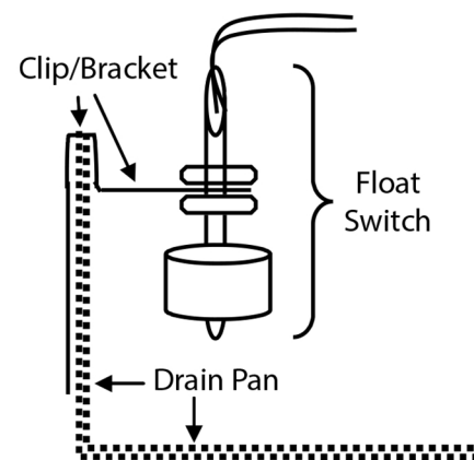
Figure 1: Installation on drain pan
